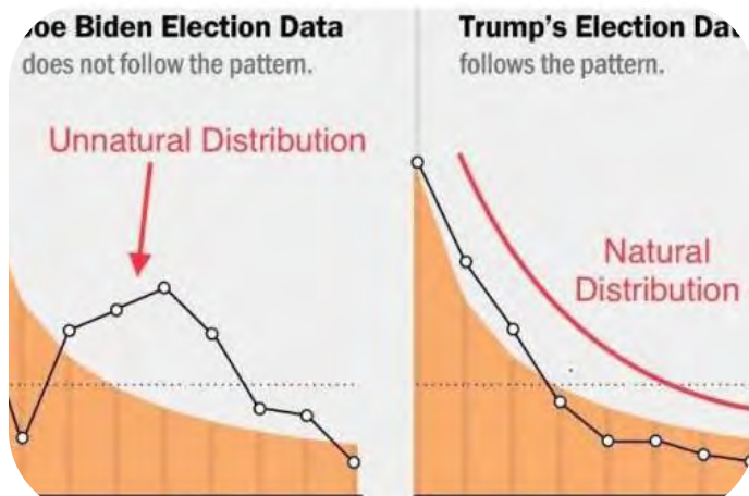
Benford's Law
